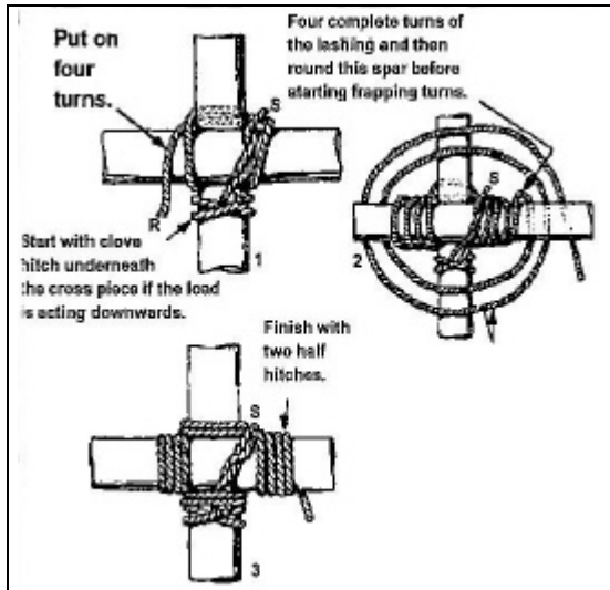
Fig 2-5-1 Square lashing
