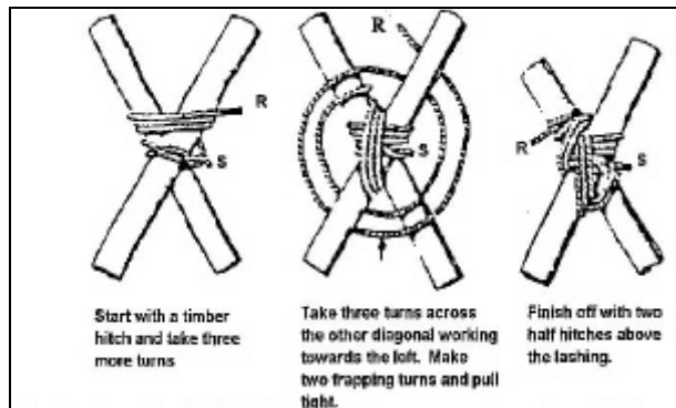
Fig 2-5-2 Diagonal lashing
