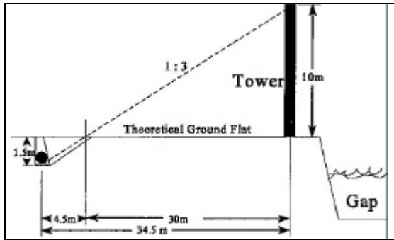
Fig 6-17 Slope ratio in level ground
