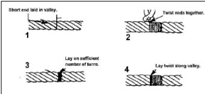
Fig 3-2-3 Whipping of steel wire ropes
