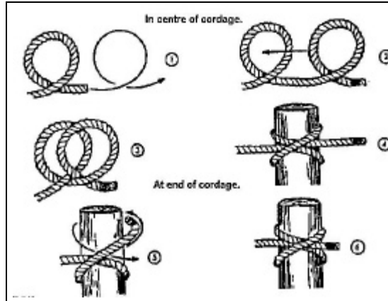
Fig 2-3-10 Clove hitch
